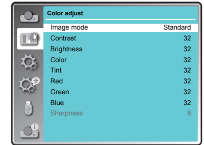
Color adjust (Video,S-video, Component)
